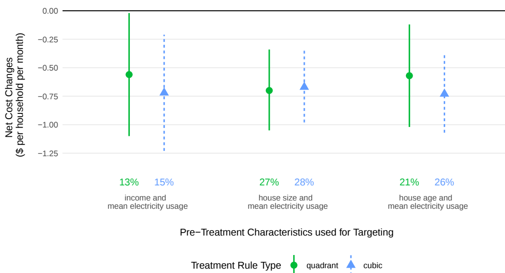
Figure 4: Estimates of the private cost savings from targeted treatment assignment
